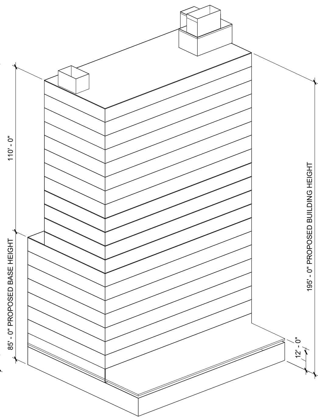
ZONING 3D VIEW II
