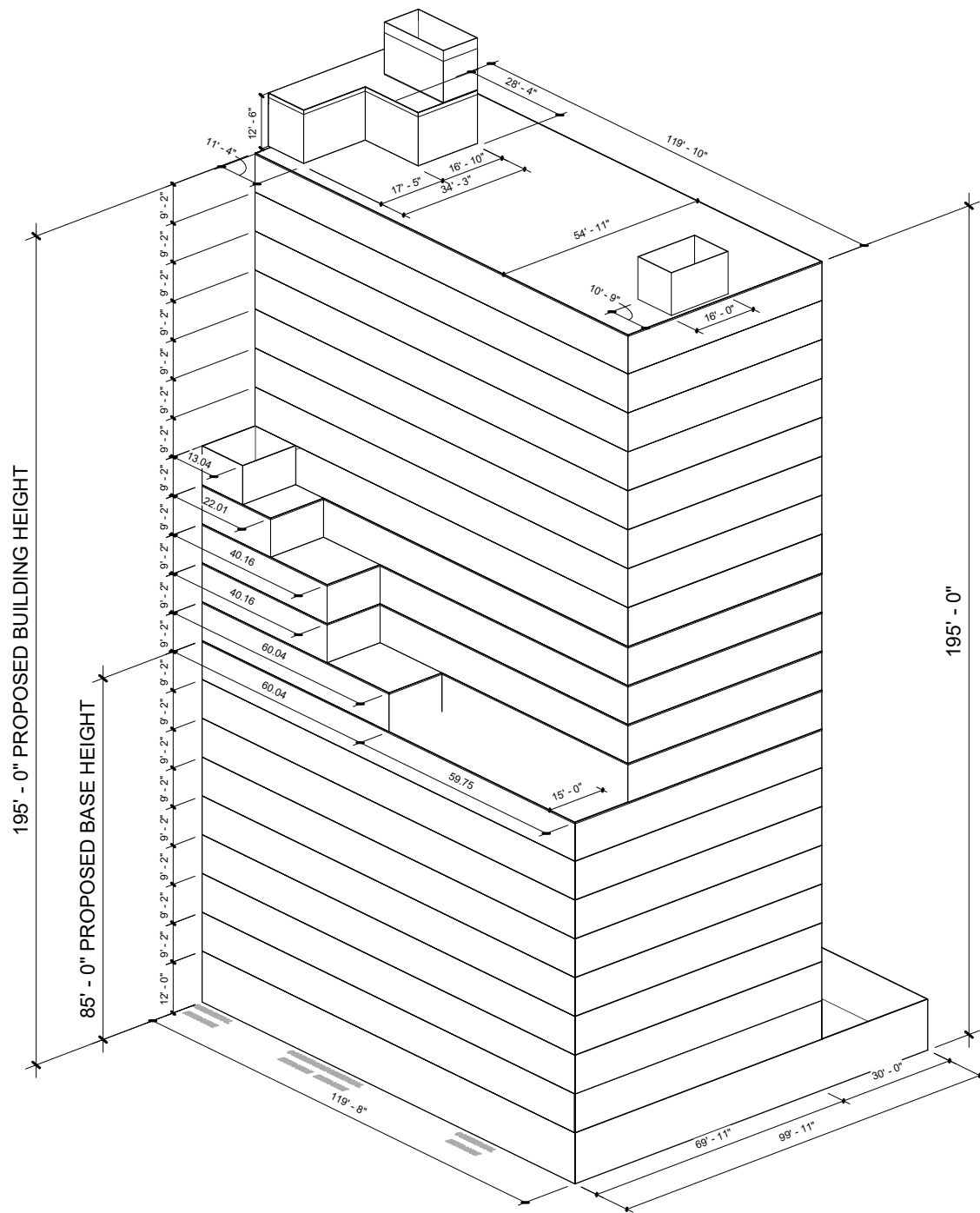
ZONING 3D VIEW I
