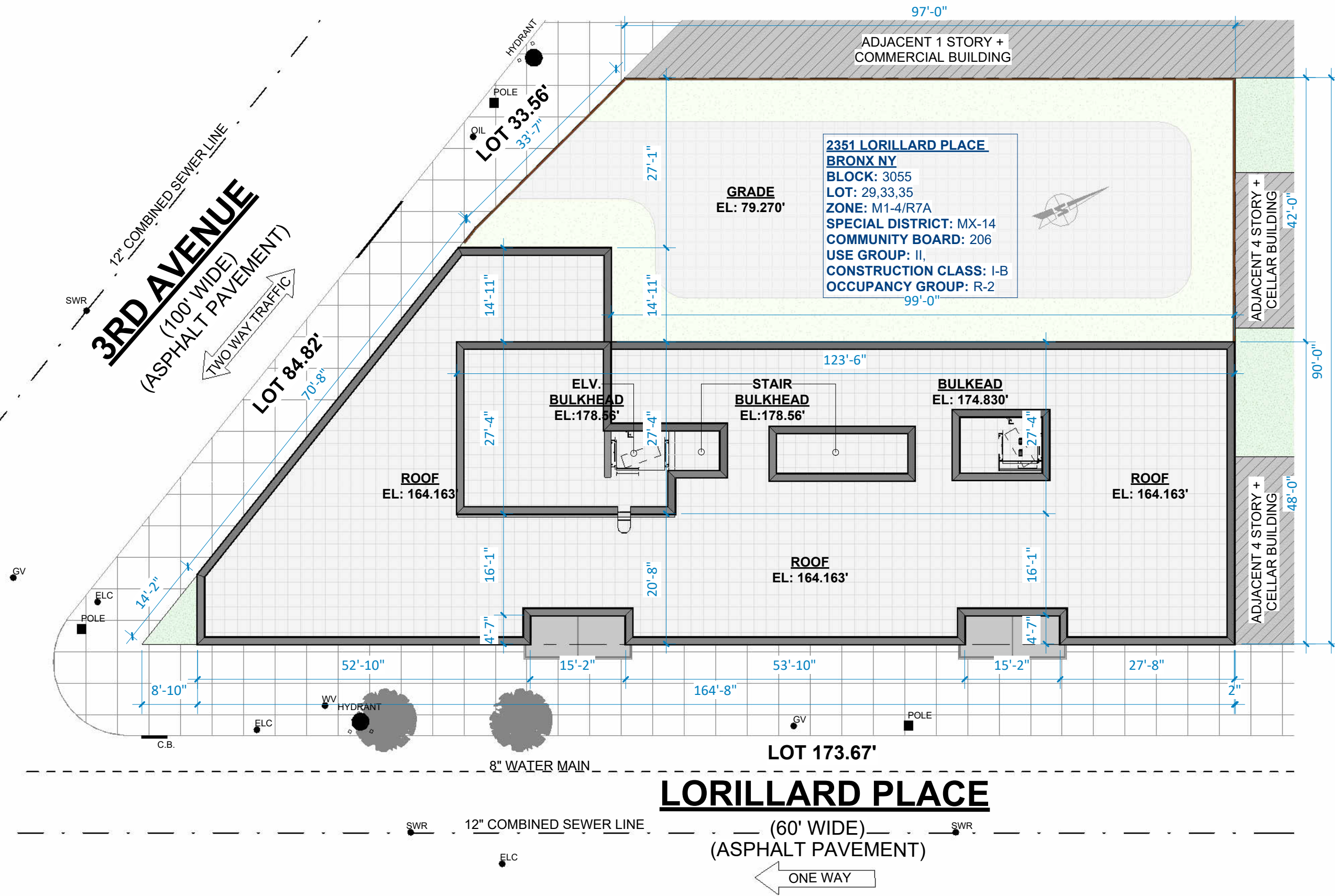
1 PLOT PLAN - ZD1 1/16" = 1'-0"
