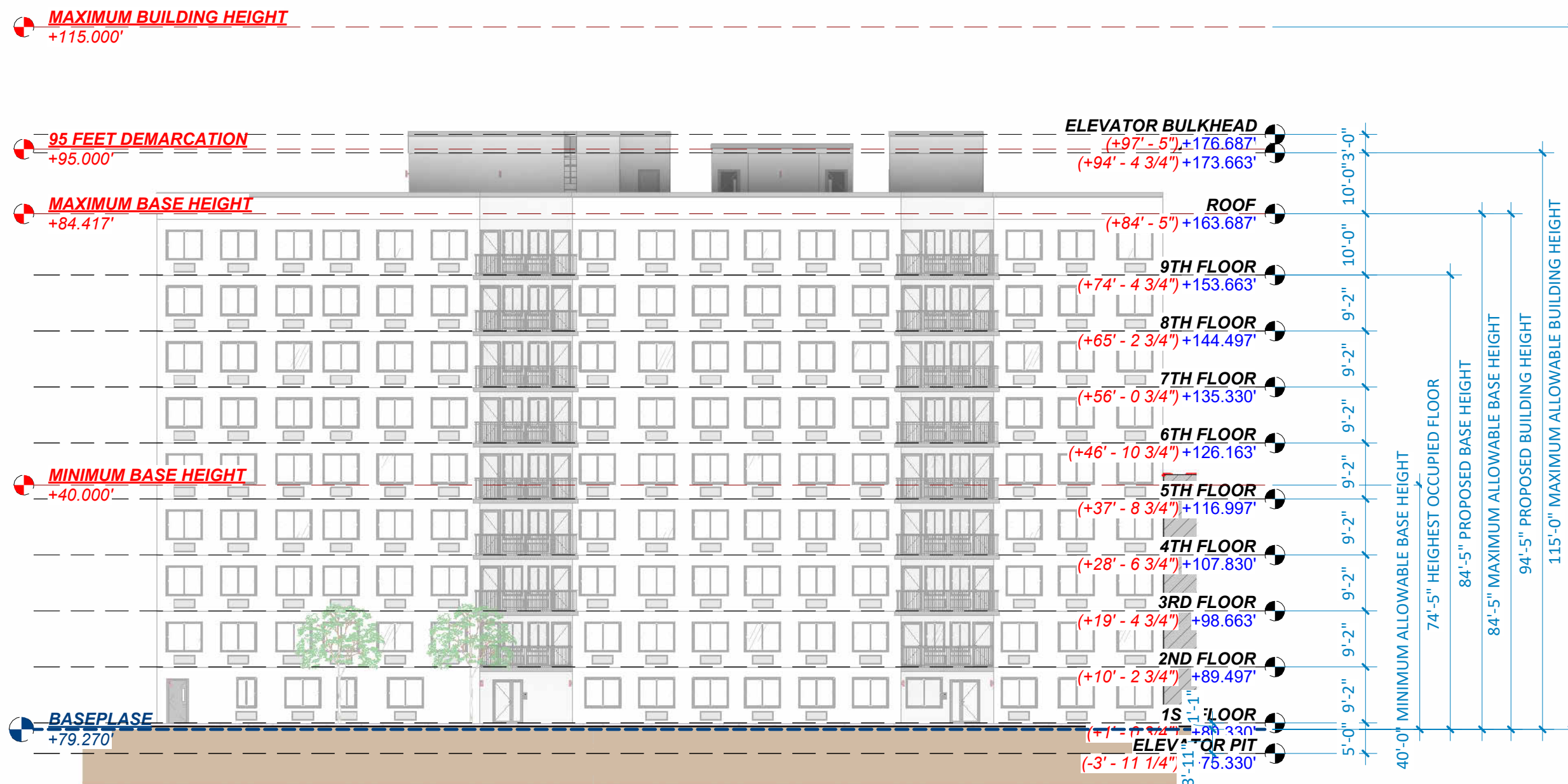
1 HEIGHT DIAGRAM - ZD1 1" = 20'-0"
