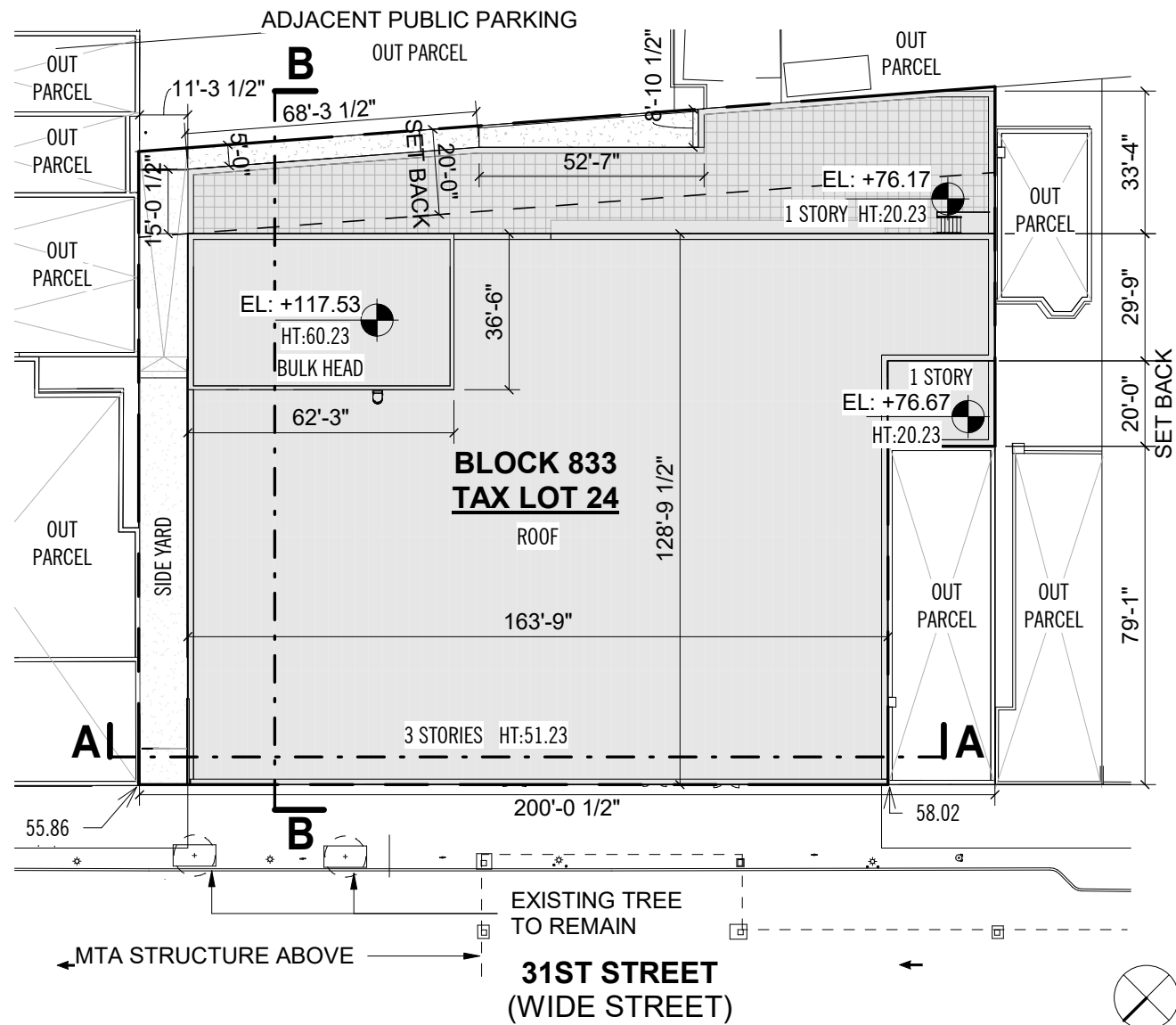
1 ZD-1 SITE PLAN DIAGRAM 1" = 40'-0"
