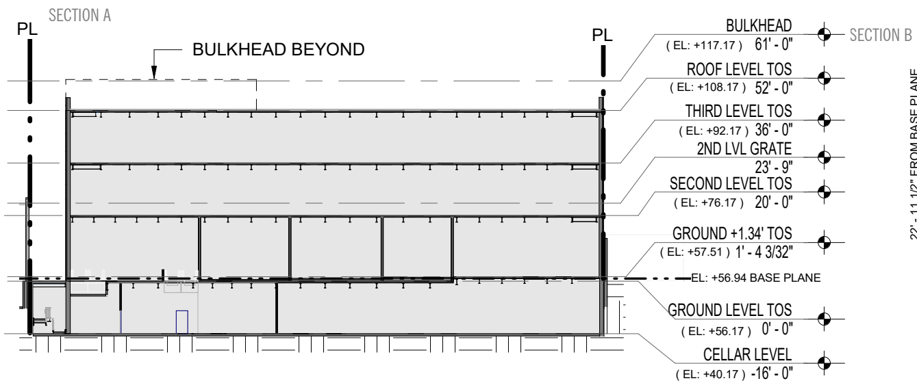
3 SECTION DIAGRAM 1" = 40'-0"
