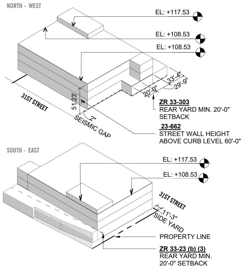
2 AXONOMETRIC DIAGRAM
