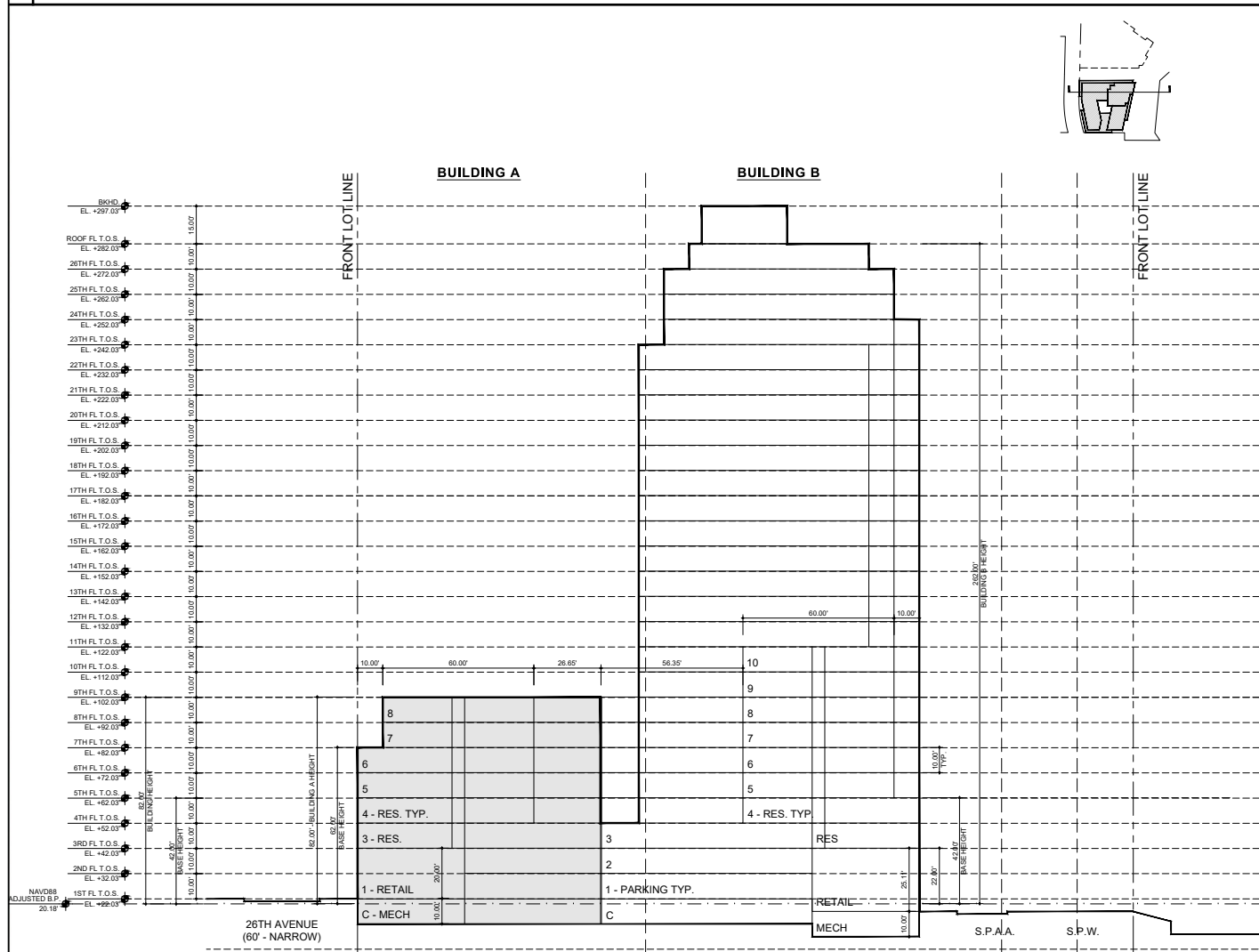
1 SITE DIAGRAM SCALE: NTS
