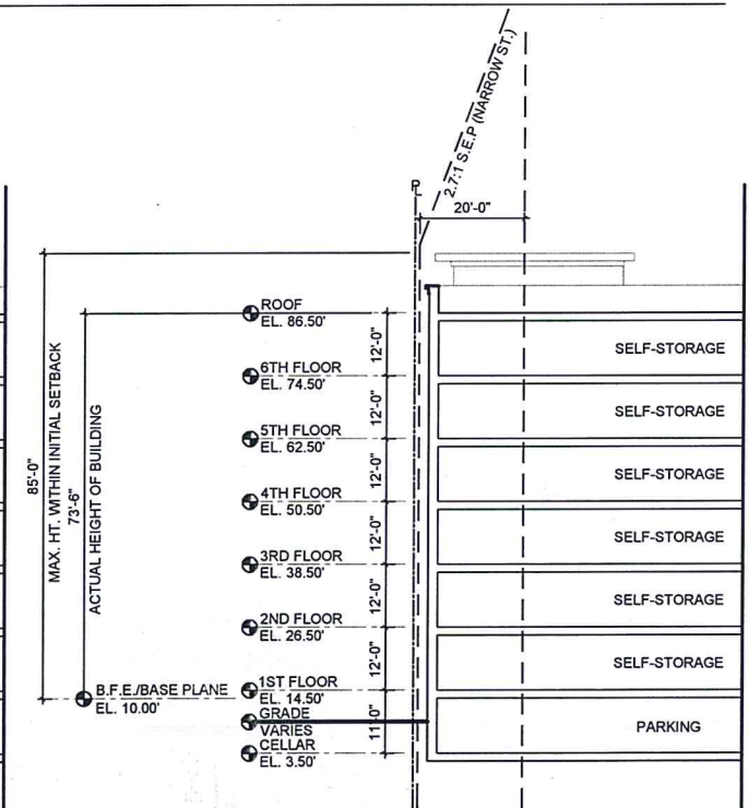
SECTION DIAGRAM (BEACH 106TH ST.)
