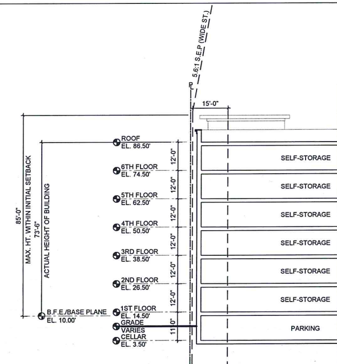
SECTION DIAGRAM (ROCKAWAY BEACH BLVD.)
