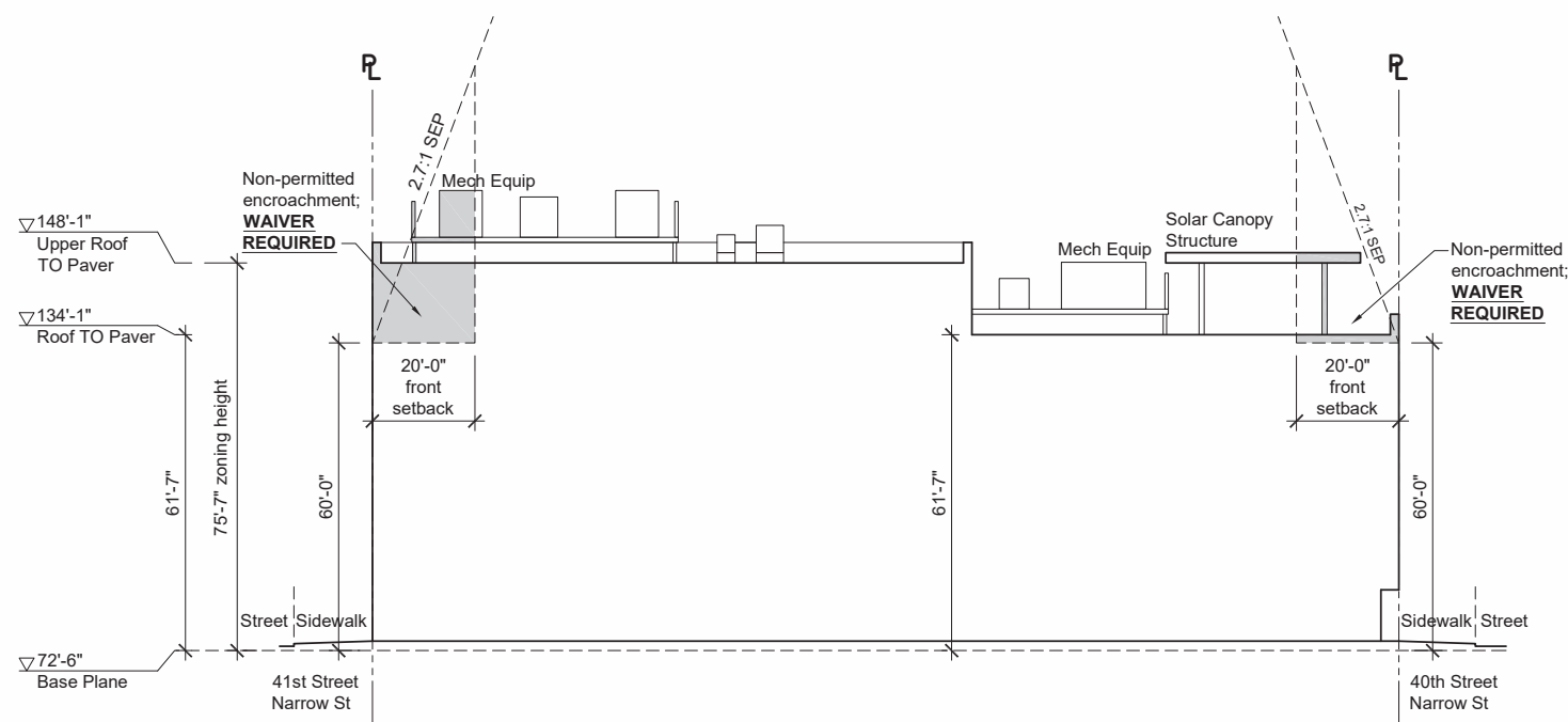
3 Zoning Section Looking North
