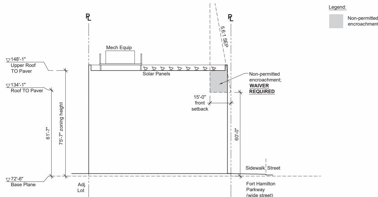
4 Zoning Section Looking East
