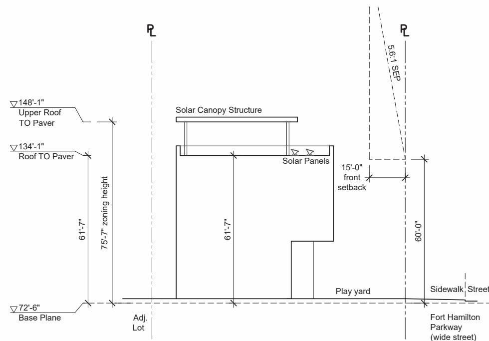
7 Zoning Section Looking East
