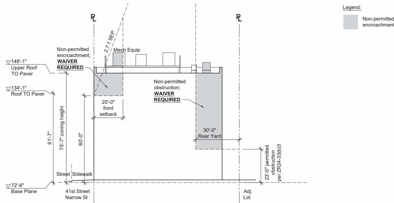
2 Zoning Section Looking North
