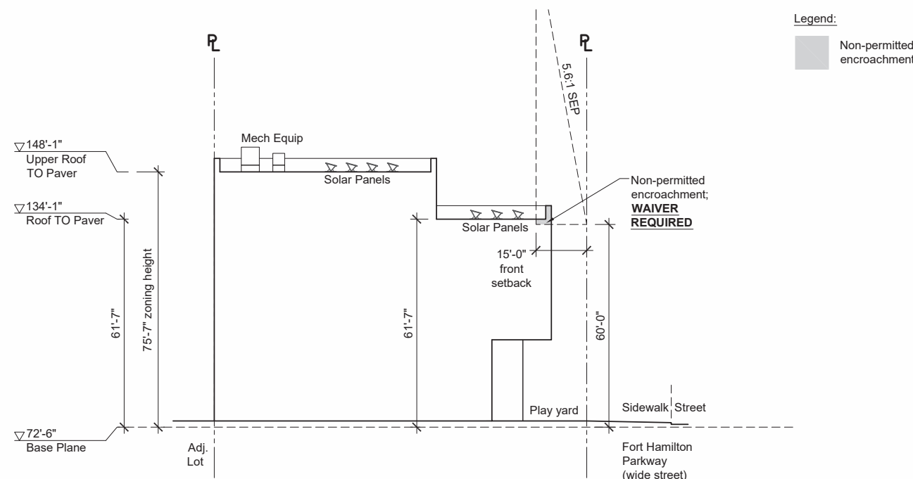
6 Zoning Section Looking East
