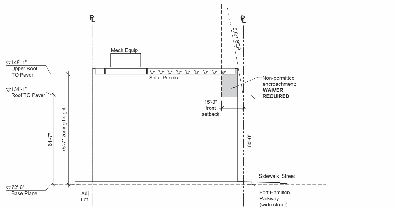
5 Zoning Section Looking East
