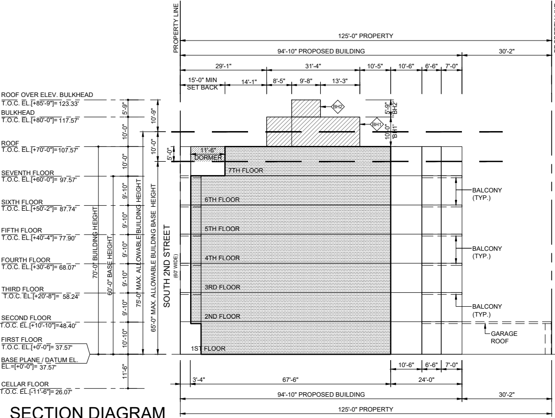
SECTION DIAGRAM SCALE 1/32"=1'-0"
