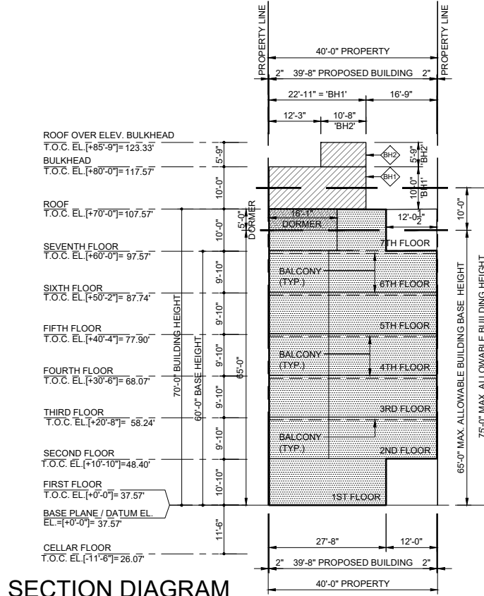
SECTION DIAGRAM SCALE 1/32"=1'-0"
