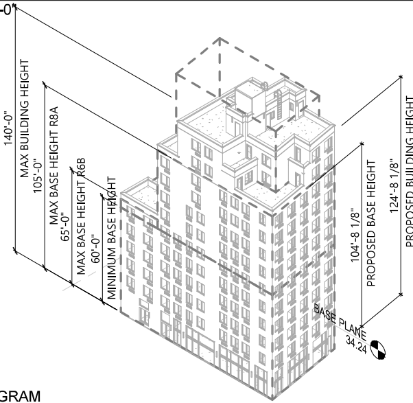
2 3D DIAGRAM
