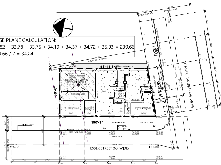
1 PLOT PLAN 1" = 40'-0"
