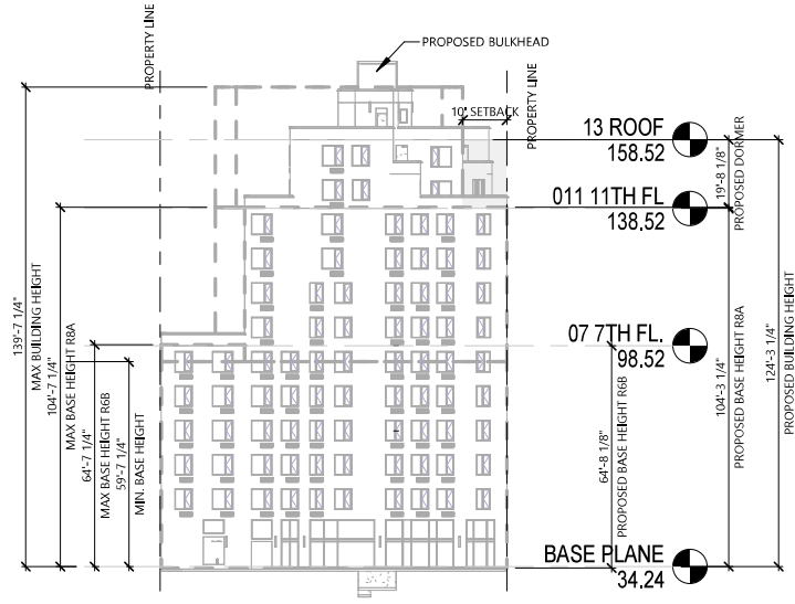
4 ESSEX STREET HEIGHT & SETBACK DIAGRAM 1" = 40'-0"
