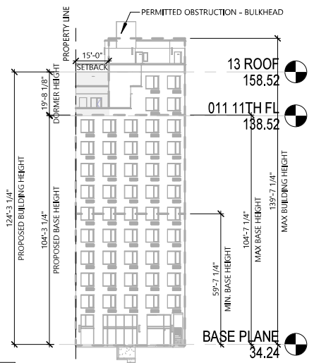
3 ATLANTIC AVE HEIGHT & SETBACK 1" = 40'-0"
